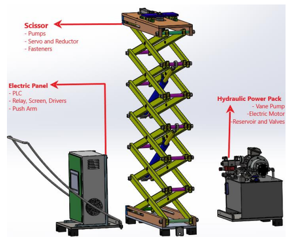
Figure 3 : 3D Model of the Scissor Subsystem
