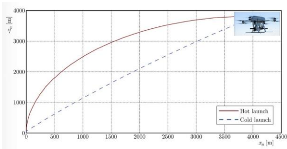
Figure 1: Trajectory motions of hot launch vs. cold launch [1]
