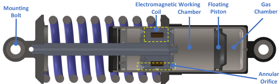
Figure 3: CAD model of the designed MR suspension system
