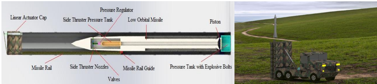
Figure 4 : 3D model Low orbital missile cold launch system
