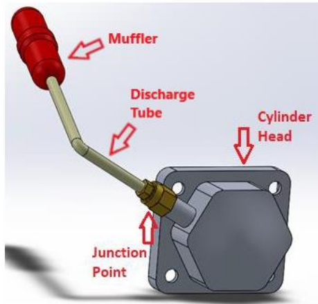
Figure 3 : 3D Inner View Model of the System
