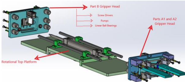
Figure 4 : CAD Model of the Rotating Top Subsystem
