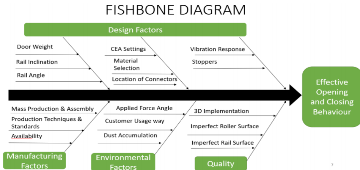
Figure 1 : The Fishbone Diagram of the Project
