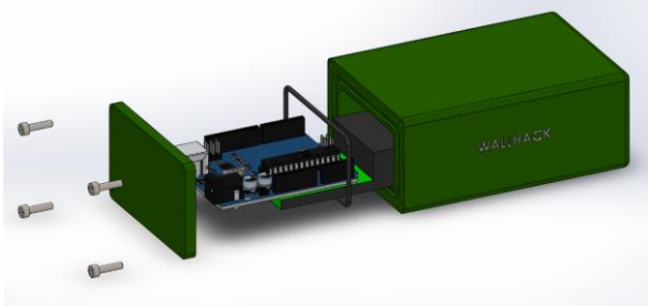
Figure 3 : Target Designation System inside housing
