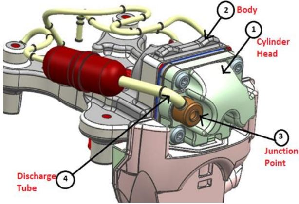
Figure 1: An inside look at components of the previous compressor design
