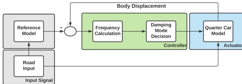
Figure 4: Schematic of the designed control system
