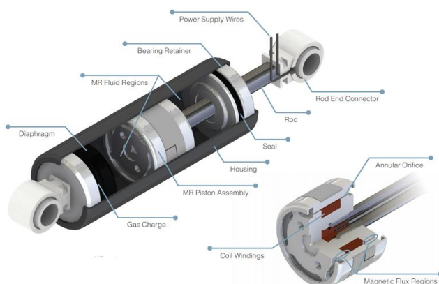
Figure 1: An exemplary MR suspension [1]
