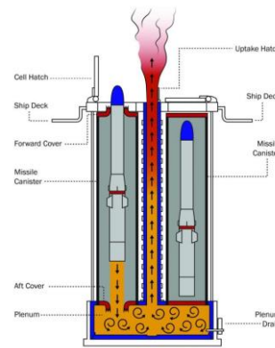
Figure 2: Hot launch of missiles [2]
