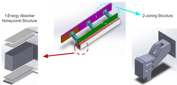
Figure 3 : 3D Model of the Proposed Design with its Components
