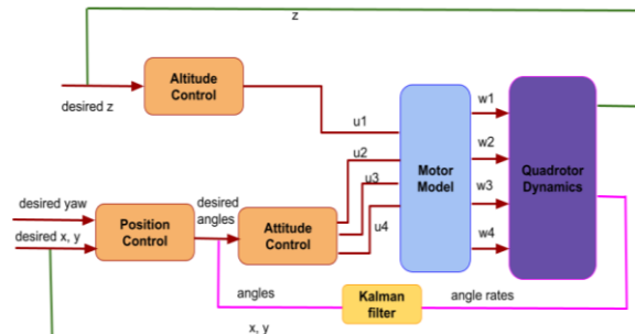
Figure 4 : Simplified Version of Quadrotor Control Algorithm
