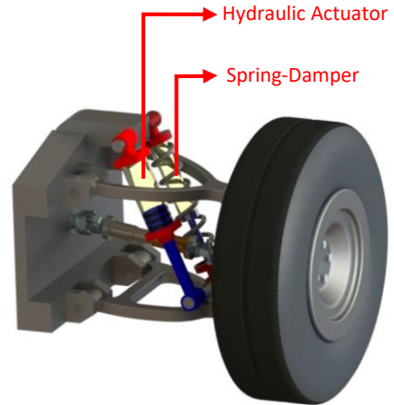
Fig. 4 : CAD Model of Quarter Car
