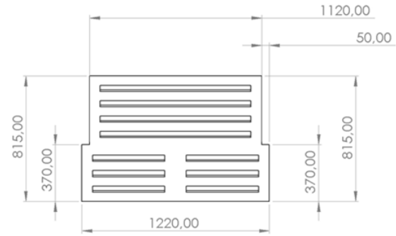
Figure 2: Dimensions of the Grill
