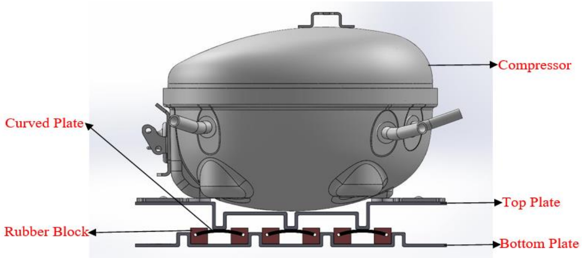
Figure 3 : Compressor and Mounting Assembly
