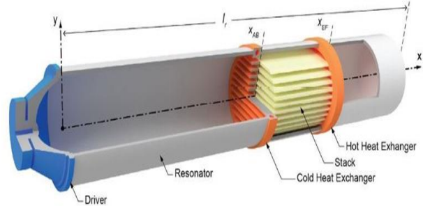
Figure 1. General Standing-Wave Thermoacoustic Refrigerator Model [1]
