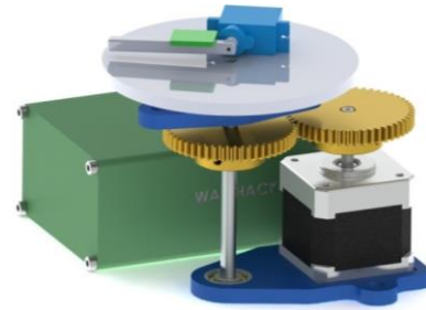
Figure 4 : Turret aiming system with its electronic components
