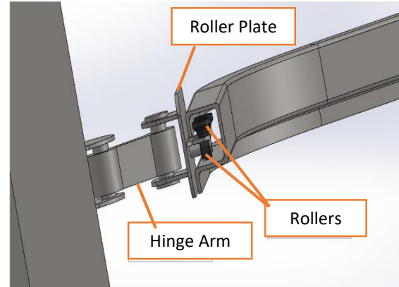
Figure 3 : Roller and Hinge Assembly
