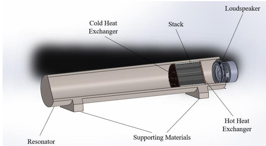
Figure 2 : 3D Model of the System
