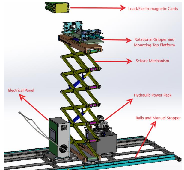
Figure 2: CAD Model of the System
