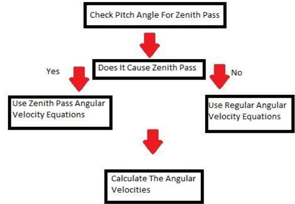
Figure 4 : The Scheme for the Control Structure
