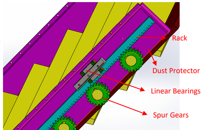
Figure 4 : Right View - 3D Model of the System
