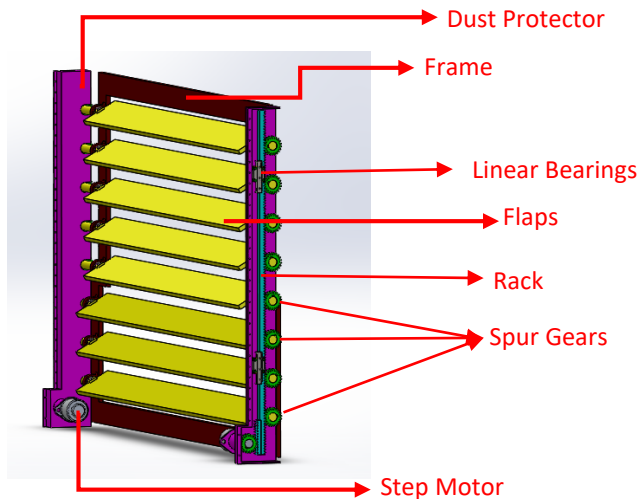
Figure 3 : 3D Model of the System
