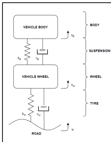
Fig. 1: Passive Suspension System for Quarter Car Model.
