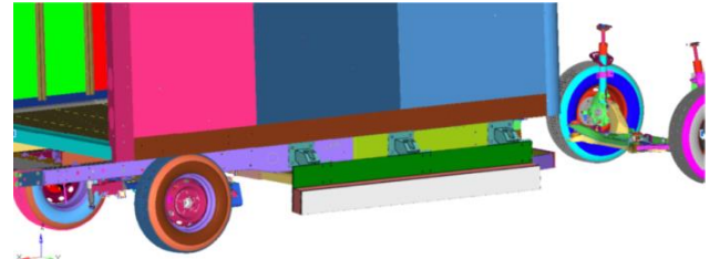
Figure 4 : The Design Location on the Ford Transit Chassis Cab (One other on the other side)
